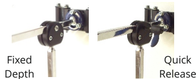
Thru Block
